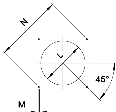
Fig. 7 Boiler plate
