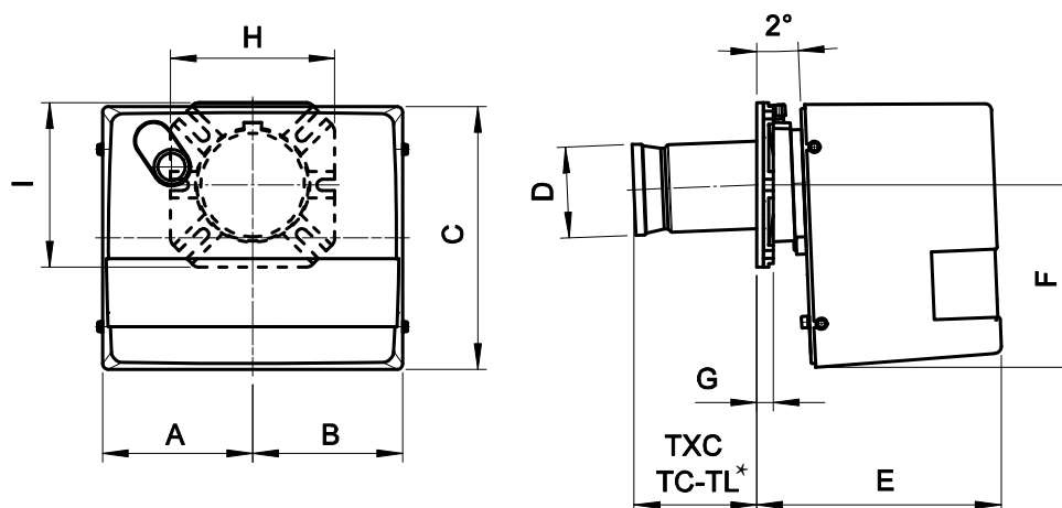
Fig. 4 Dimensions G 0HR - G 0SR - G 0H - G 0S - G 1HR - G 1SR - G 1H - G 1S
