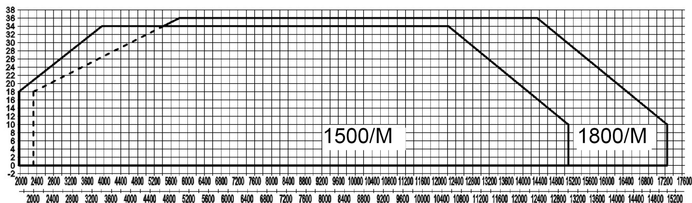
Fig. 2 X = Thermal power [kg/h - Mcal/h] Y = Pression in the combustion
