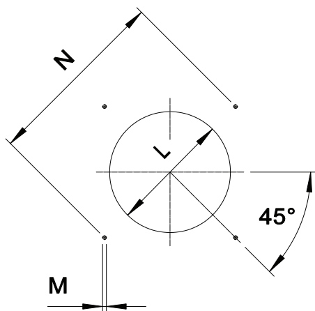
Fig. 4 Boiler plate
