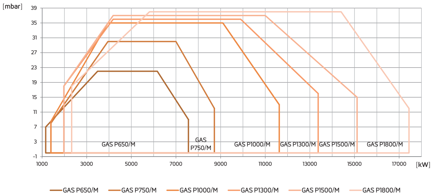
Fig. 2 X = Thermal power [kW] Y = Pression in the combustion
