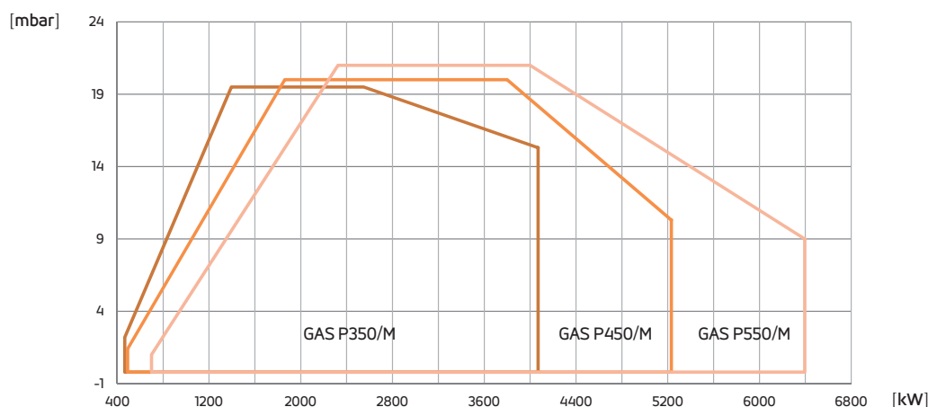
Fig. 6 X = Thermal power Y = Pression in the combustion chamber
