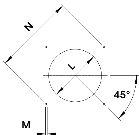
Fig. 8 Boiler plate
