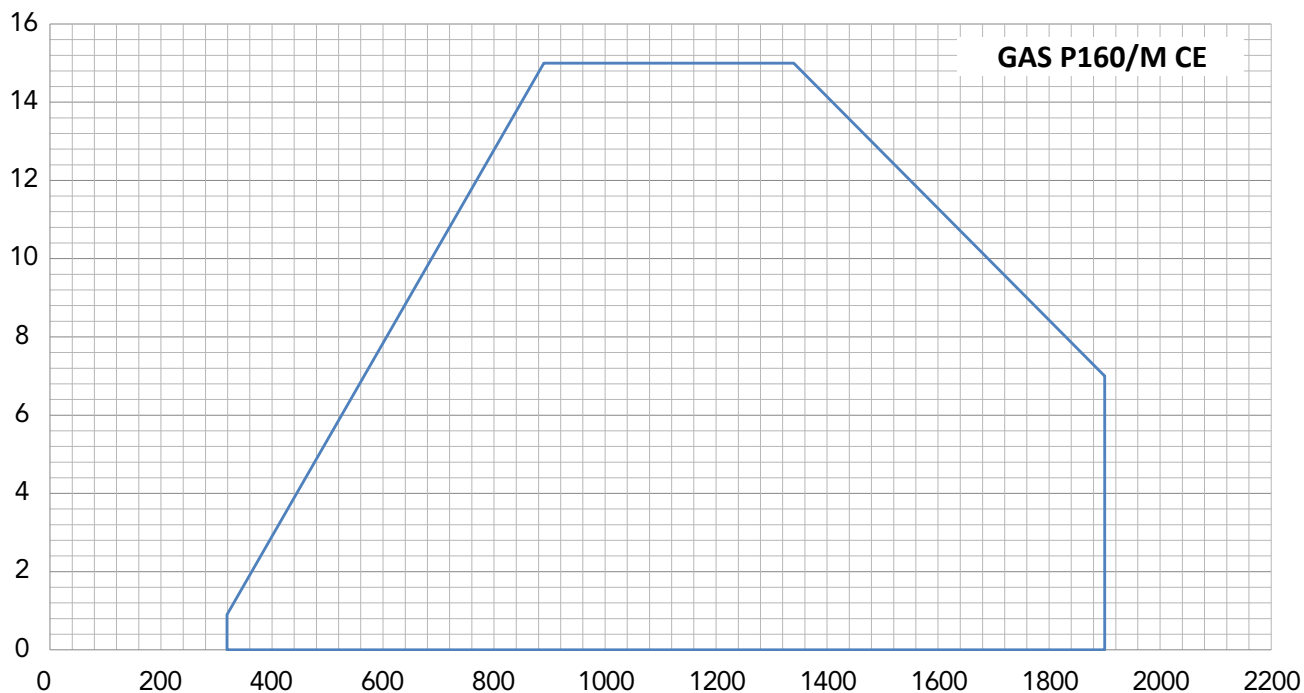
Fig. X = Thermal power [kW] Y = Pressure in the combustion chamber [mbar]
