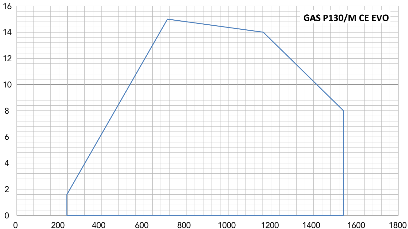
Fig. X = Thermal power [kW] Y = Pressure in the combustion chamber [mbar]
