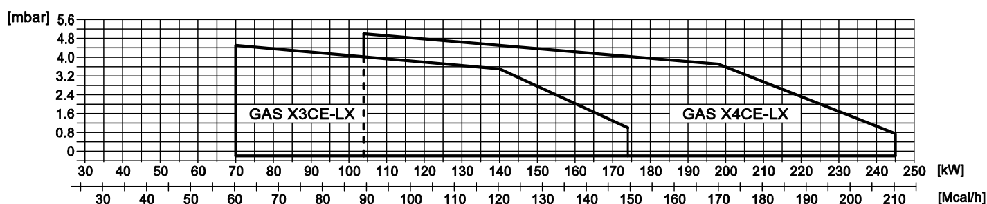
Fig. 3 X = Thermal power Y = Pression in the combustion chamber
