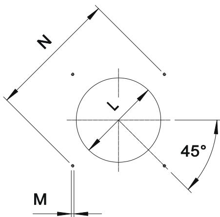
Fig. 5 Boiler plate
