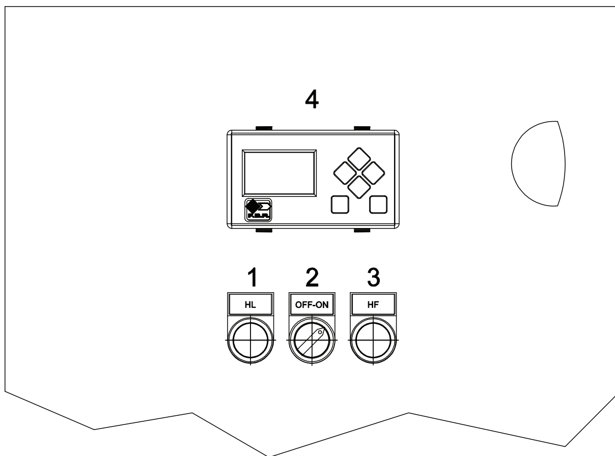
Fig. 5 Burner control panel
